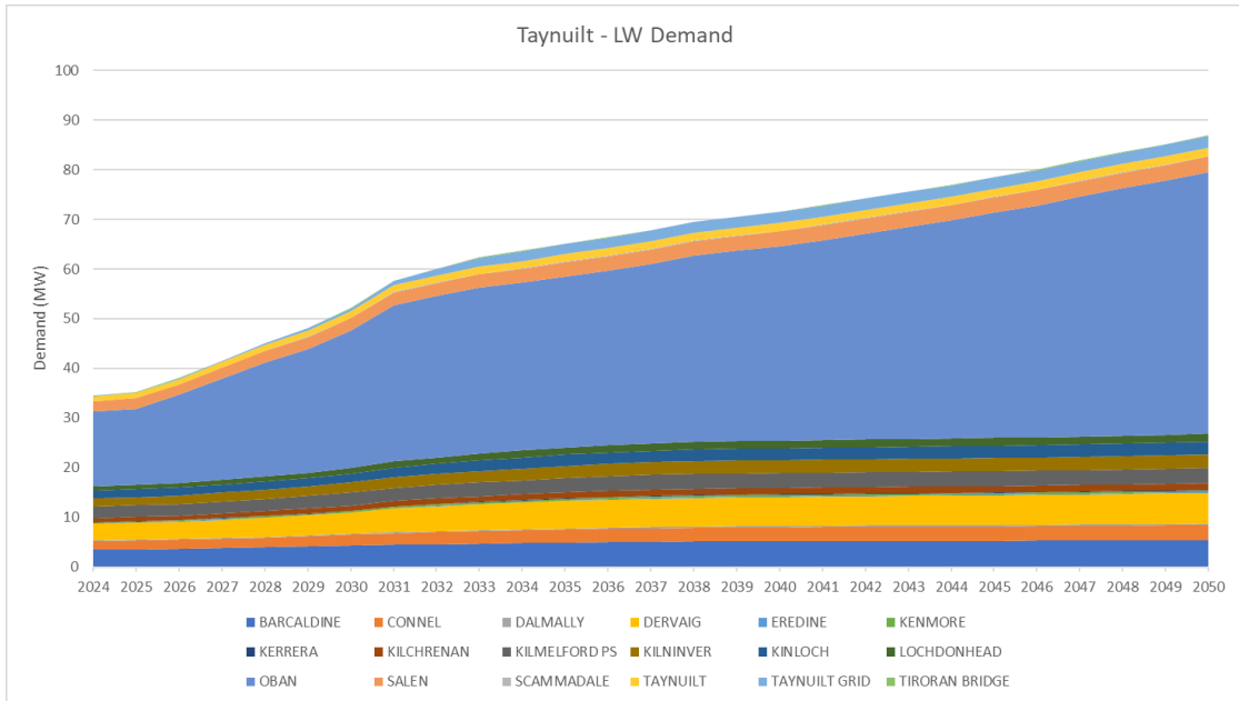
Figure 39 Demand Forecast for Taynuilt – Breakdown by Primaries - LW Source: SSEN DFES 2023
