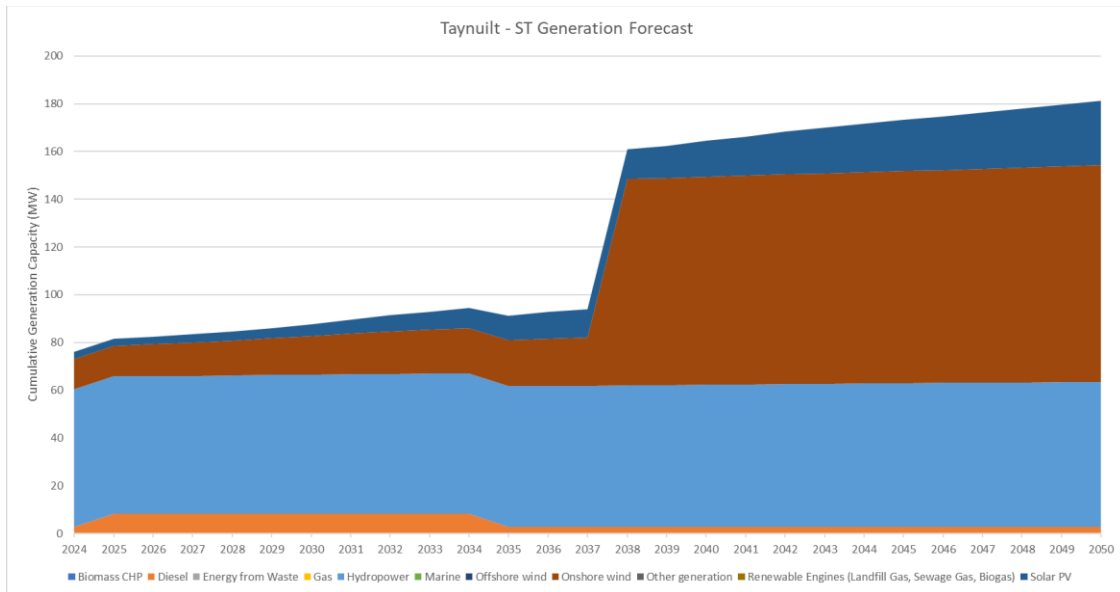
Figure 34 Cumulative Generation Forecast Breakdown by Technology for Taynuilt – ST Source: SSEN DFES 2023
