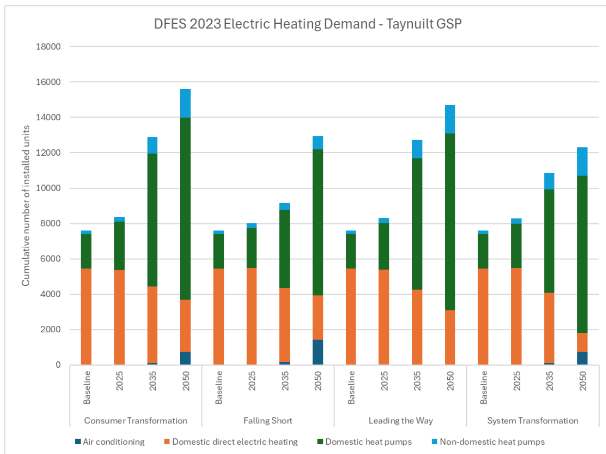
Figure 12 Projected number of Heat Pumps across Taynuilt GSP group. Source: SSEN DFES 2023
