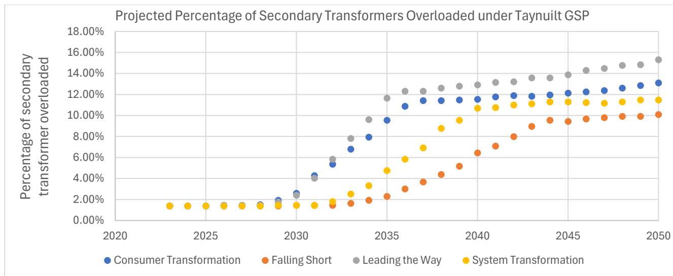
Figure 32 Taynuilt Projected Secondary Transformer Loading. Source: SSEN Load Model
