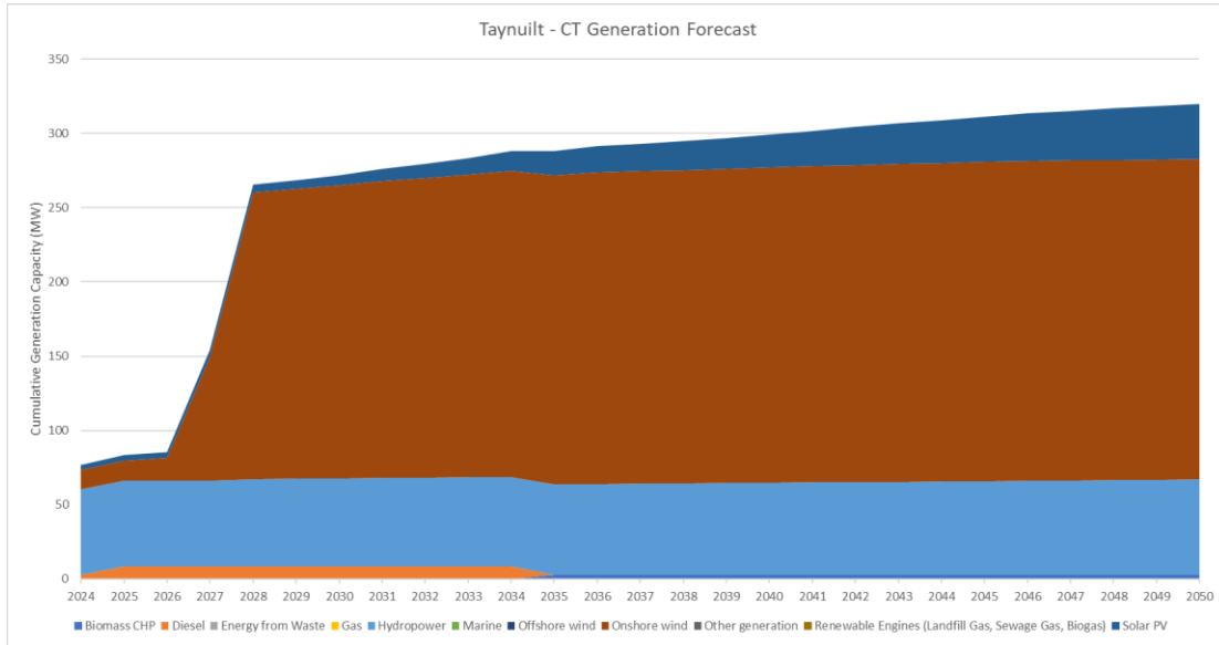
Figure 33 Cumulative Generation Forecast Breakdown by Technology for Taynuilt – CT Source: SSEN DFES 2023
