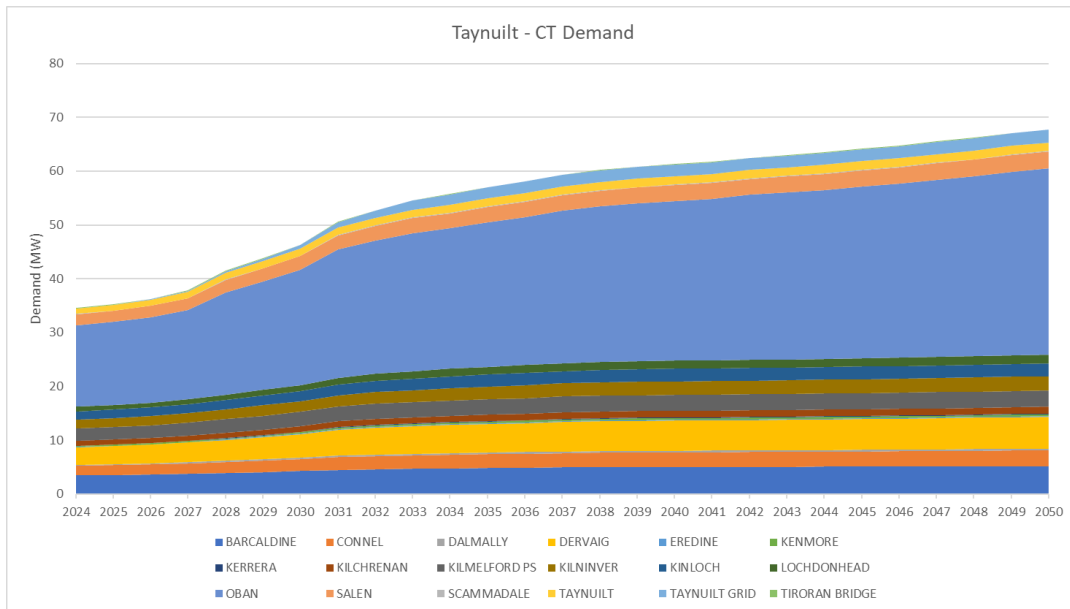
Figure 37 Demand Forecast for Taynuilt – Breakdown by Primaries - CT Source: SSEN DFES 2023
