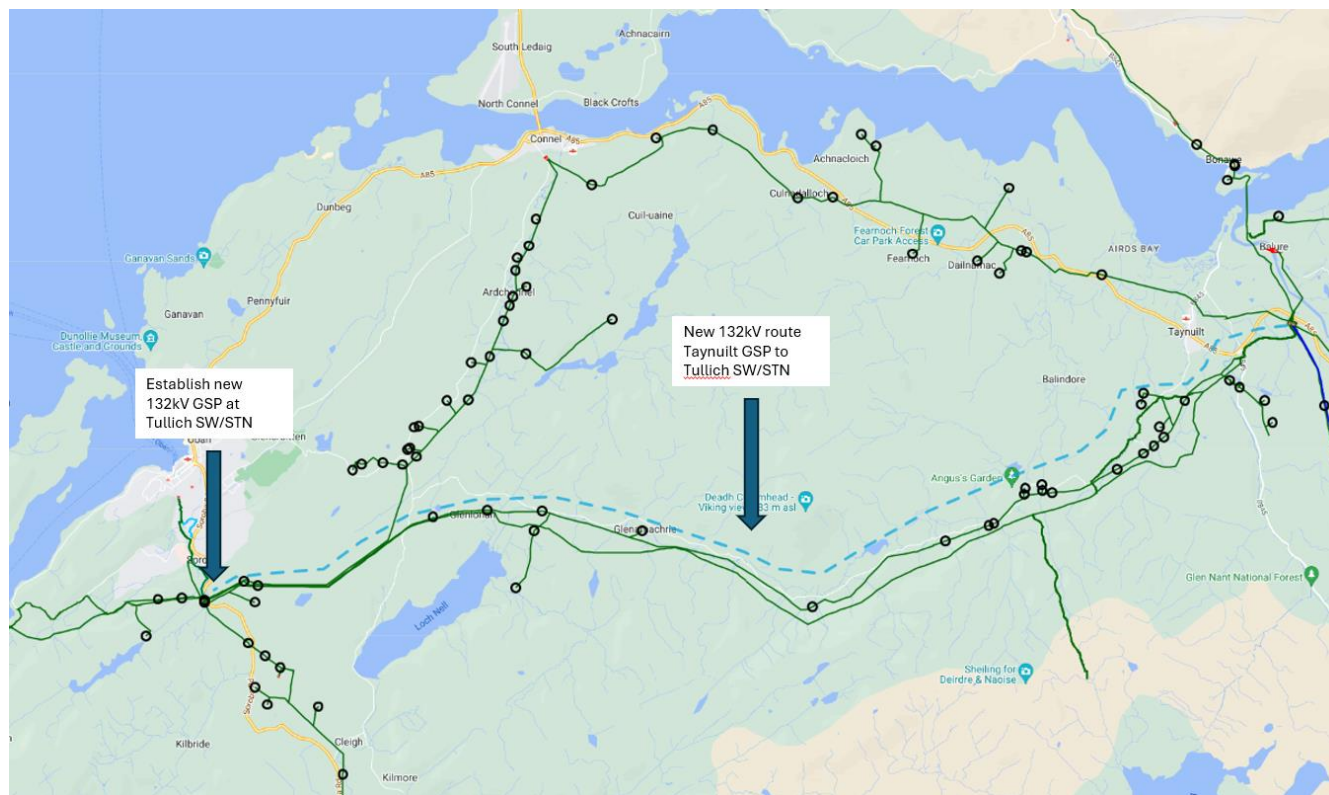
Figure 31 Network schematic with system needs 2029-2035 – Upgrading Tullich SW/STN to 132kV
