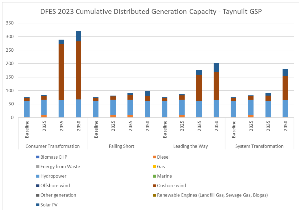
Figure 9 Projected Cumulative Distributed Generation Capacity Taynuilt GSP (MW). Source: SSEN DFES 2023
